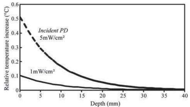
Fig. 7. Temperature increments for a homogeneous skin model exposed to a plane wave at 60 GHz.
