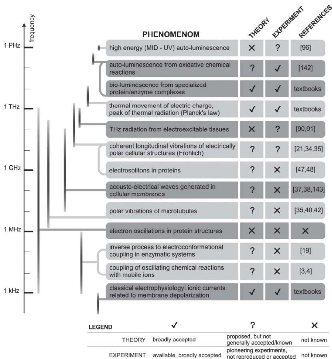
Fig. (2). A detailed distribution of the bio-electromagnetic phenomena within the electromagnetic spectrum. If the experiments proposed to confirm the theory mentioned in the text were only indirect or not giving mechanistic explanation we do not consider them in this figure.
